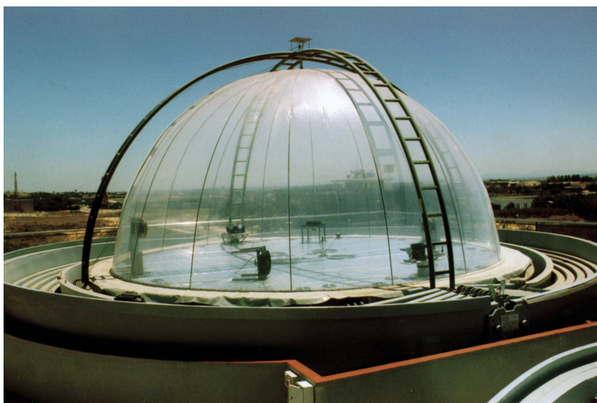
The European Photoreactor (EUPHORE) at CEAM, Valencia, Spain
